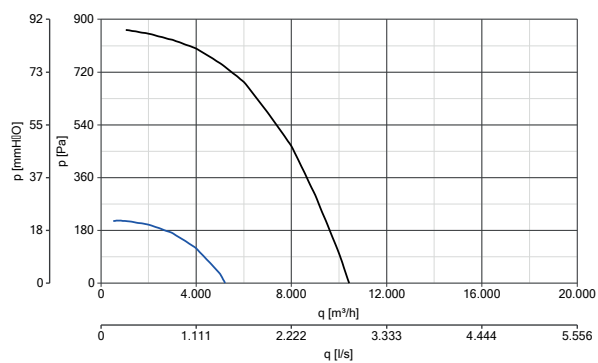
HEATMASTER F400 500 T4/8 1,5/0,25KW 80°C codice 15330
