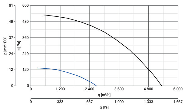
HEATMASTER F400 400 T4/8 0,75/0,12KW 80°C codice 15328
