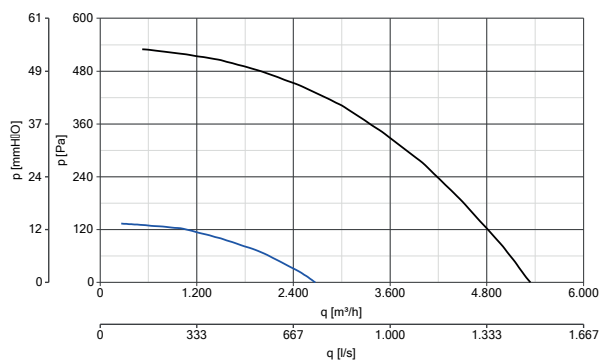
HEATMASTER F400 400 T4/8 0,75/0,12KW 120°C codice 15306
