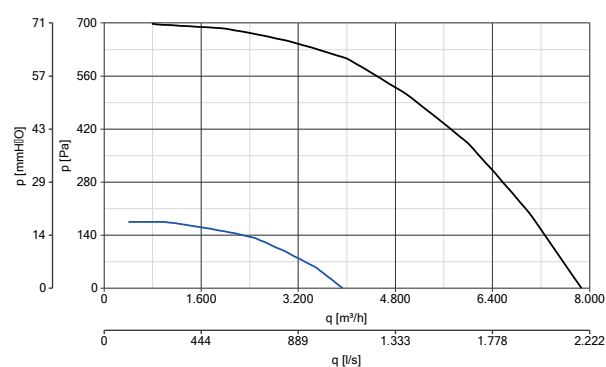
HEATMASTER F400 450 T4/8 1,1/0,18KW 120°C codice 15307
