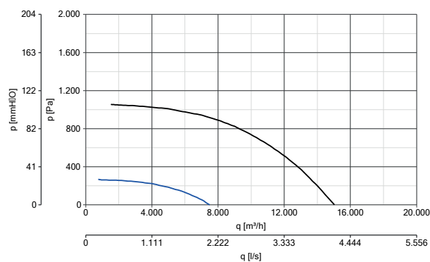
HEATMASTER F400 560 T4/8 3/0,55KW 80°C codice 15331
