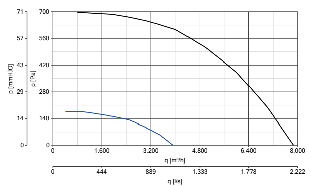
HEATMASTER F400 450 T4/8 1,1/0,18KW 80°C codice 15329
